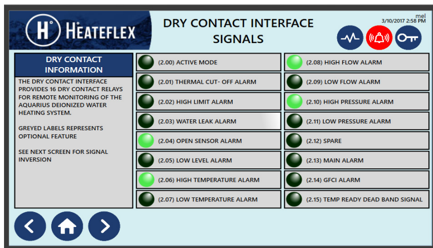
Figure 18-1: Dry Contact Interface Signals Screen #1
