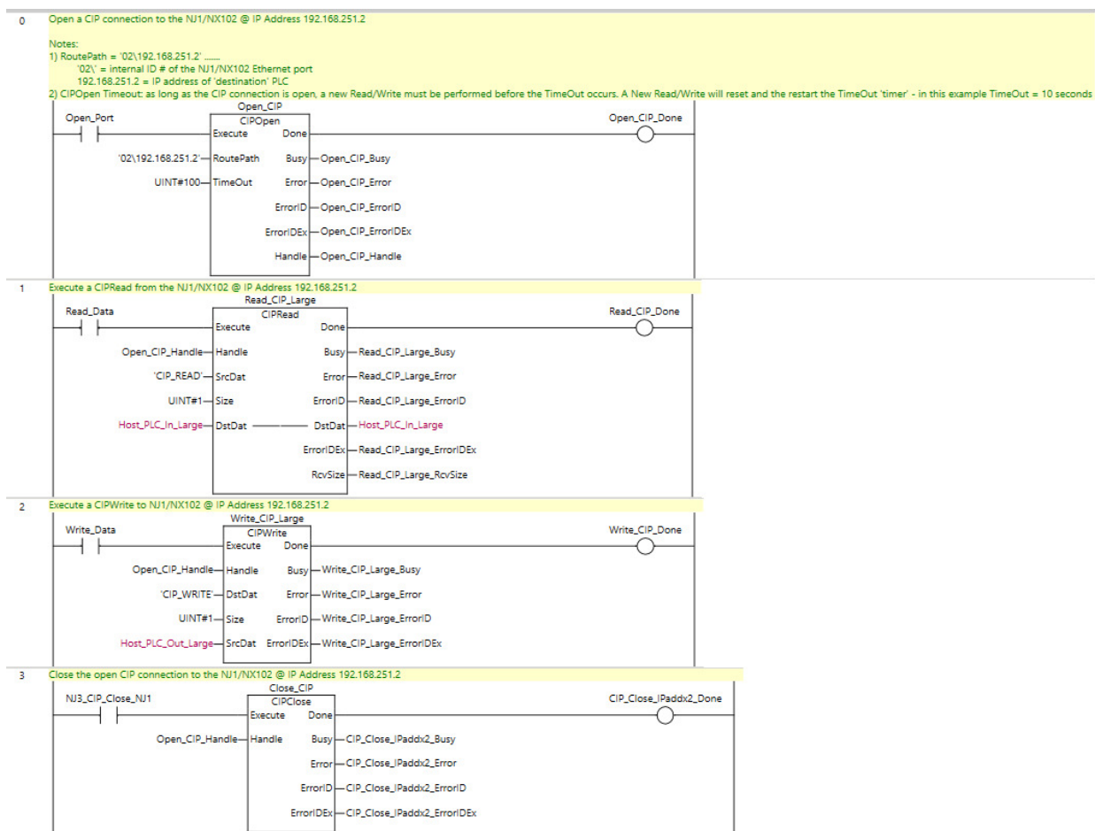
Figure 11-2 – Host Omron PLC Sample Code for Communicating PLC to PLC via Ethernet
